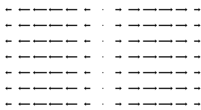
i / An impossible wave pattern.
